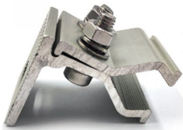
Photovoltaic Solar Beginning Clamp
